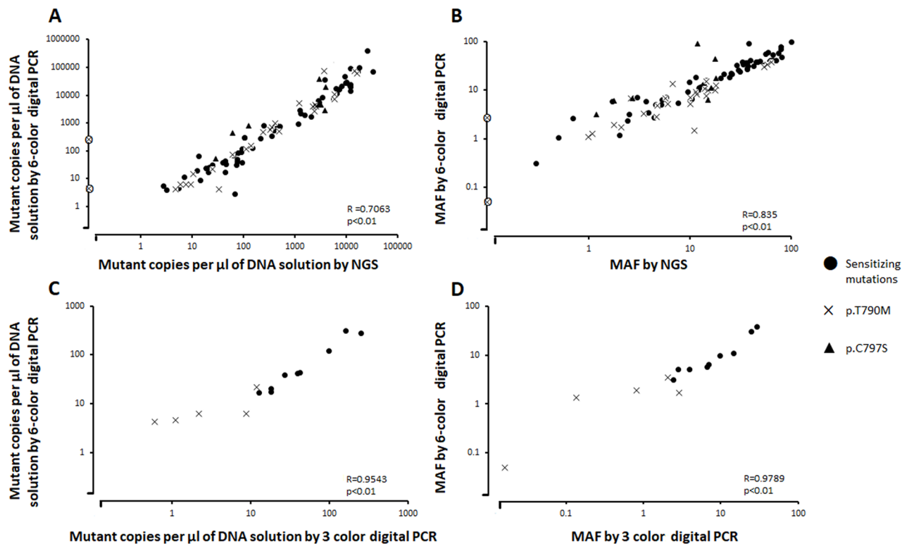
Figure 2: (A) Number of copies per \mu\text{l} of DNA solution and (B) Mutant allele fraction (MAF, %) of EGFR sensitizing and resistance mutations in tumor and plasma samples of NSCLC patients measured by 6 color digital PCR and by NGS. (C) Number of copies per \mu\text{l} of DNA solution and (D) MAF (%) of EGFR sensitizing and resistance mutations in 10 plasma samples measured by 3 color and 6 color digital PCR. Additional “o” mark in A) and B): EGFR T790M mutation detected by the 6-color digital PCR assay but not detected by NGS.
